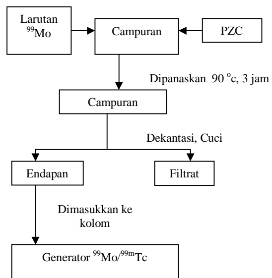
Gambar 1. Skema perakitan Generator ^{99}\text{Mo}/^{99\text{m}}\text{Tc} berbasis PZC
